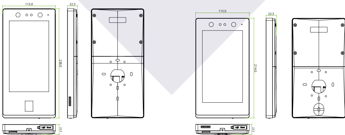
SenseFace 7A
